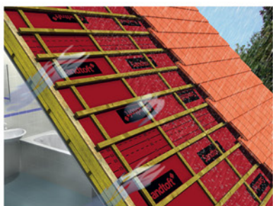
Koratech® Classic & Koratech® Classic Super Vapour permeable membranes suitable for both warm and cold roof designs on any roof shape and building type.
